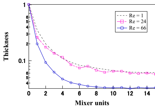
Fig. 7 Average thickness of fluid layer in various Reynolds numbers.
